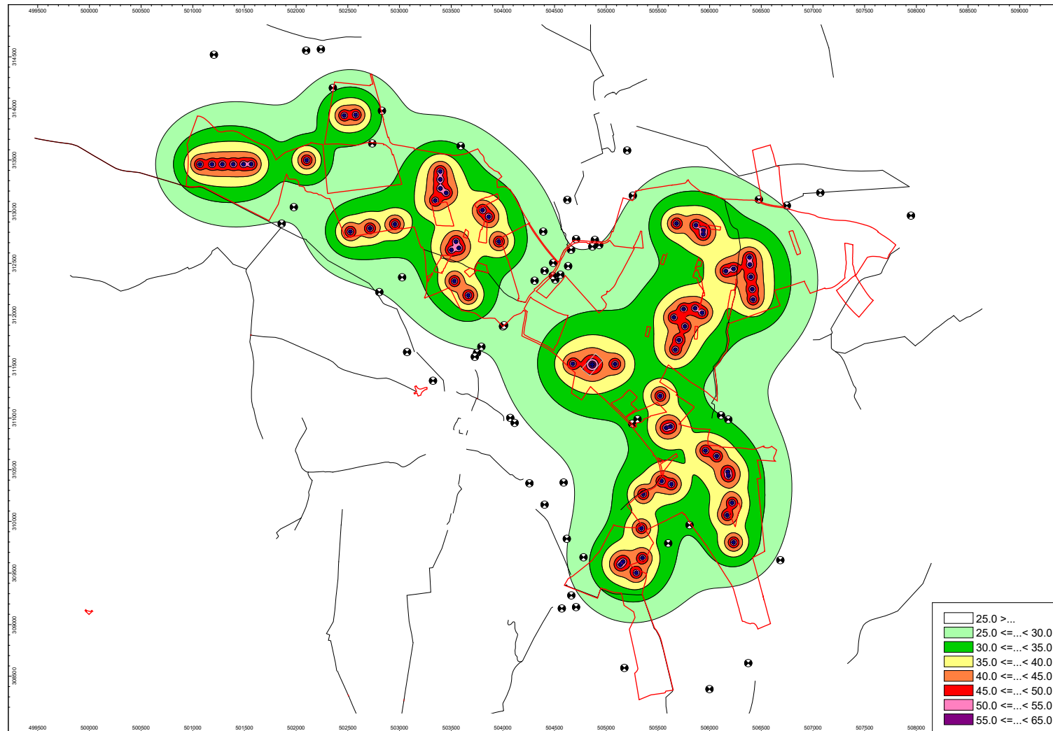
Figure 10.5.6 – Noise predictions with SAT central inverter arrangement, including receptor locations (black/white dots) and PRow (black lines)
