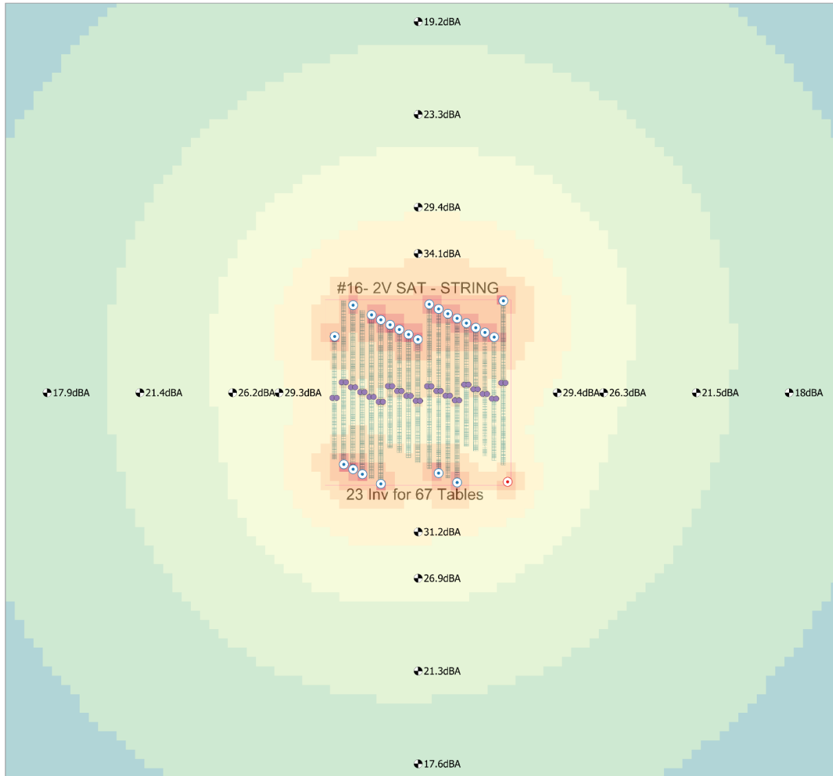
Figure 10.5.2 – calculated noise levels SAT - string inverter configuration
