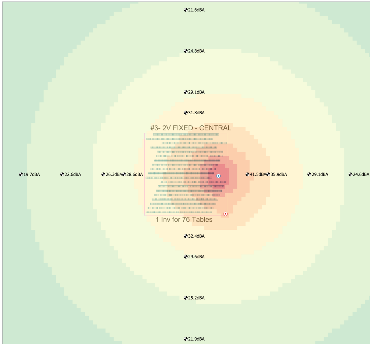
Figure 10.5.5 – calculated noise levels Fixed panels - central inverter configuration
