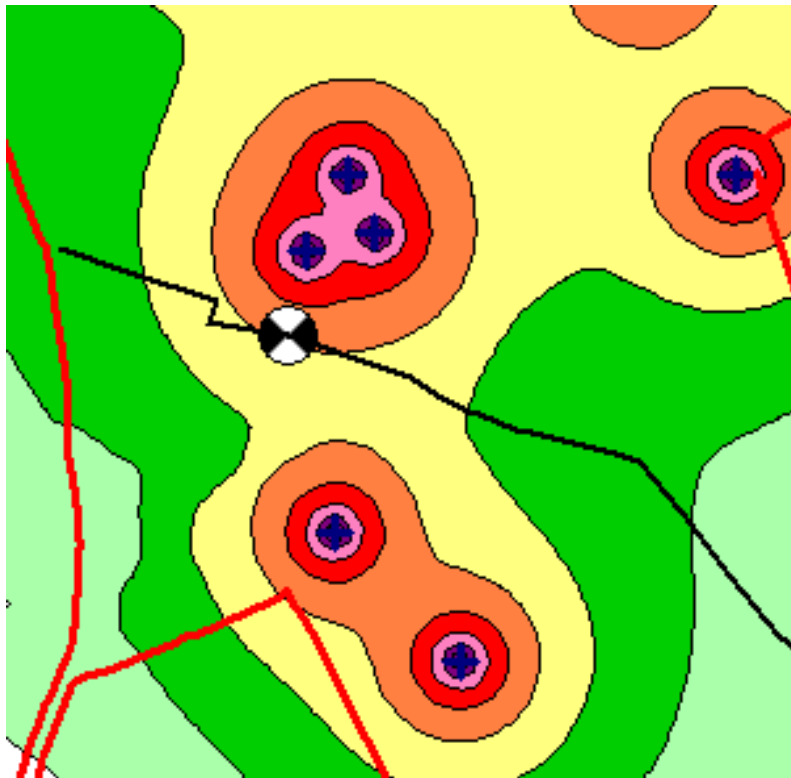
Figure 10.5.7 – Noise predictions – Close up views of Figure 10.5.6 showing the E169/1 (left image) and BrAW/1/1 (right image) PRoW paths. A representative calculation point is shown for each PRoW.
