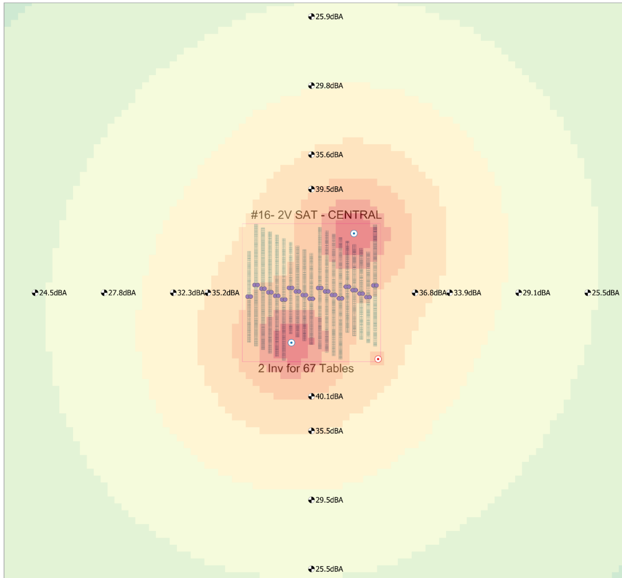
Figure 10.5.3 – calculated noise levels SAT – central inverter configuration
