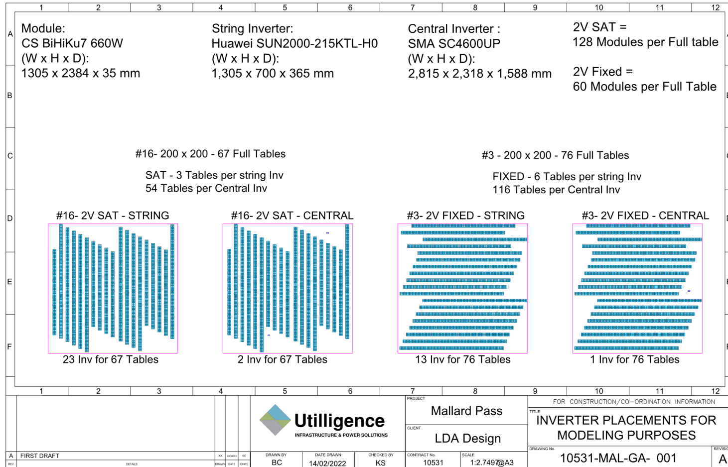
Figure 10.5.1 – sample 200 x 200 m solar PV area showing different configurations modelled
