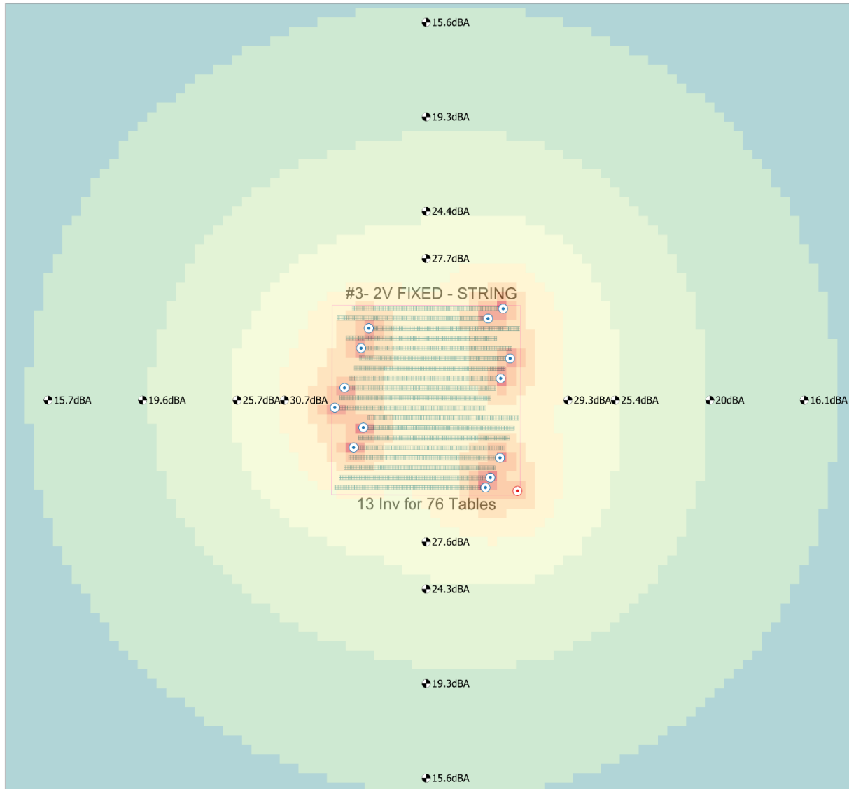
Figure 10.5.4 – calculated noise levels Fixed panels - string inverter configuration
